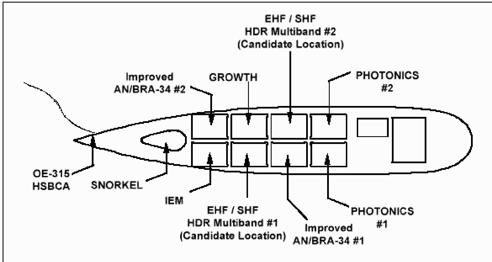
Figure A-9. New Attack Submarine Sail/Antenna Baseline Configuration
